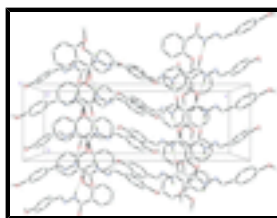
Fig. 2. The molecular packing of the title compound, viewed along the a axis. Hydrogen bonds are drawn as dashed lines.
